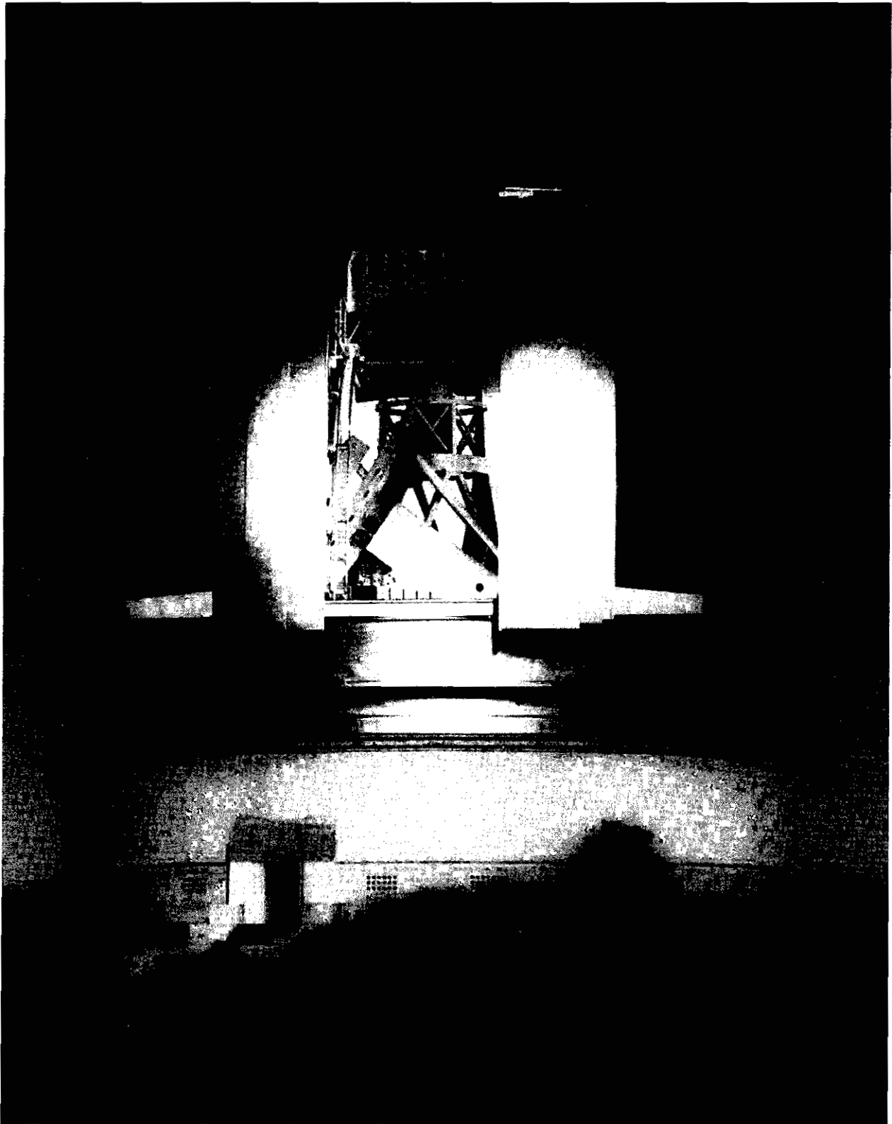
Mount Palomar Observatory, in nighttime operation.
